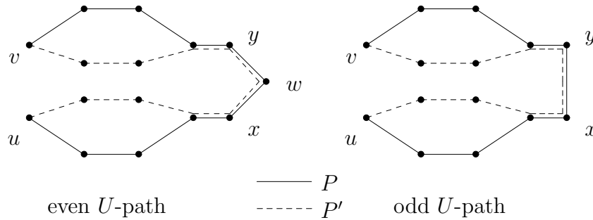
Figure 1. Two U -paths P and P' belonging to the same family \mathcal{F}(P) differ only by the shortest paths from u to x and/or from v to y that they include.
